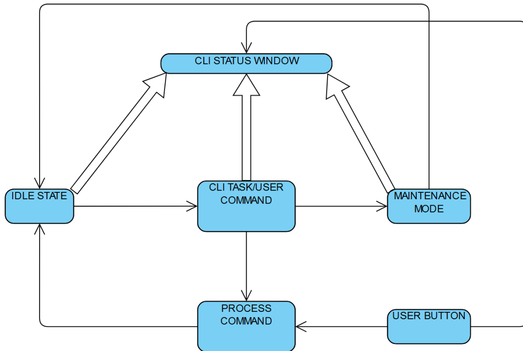
Task diagram: elevator in free rtos
